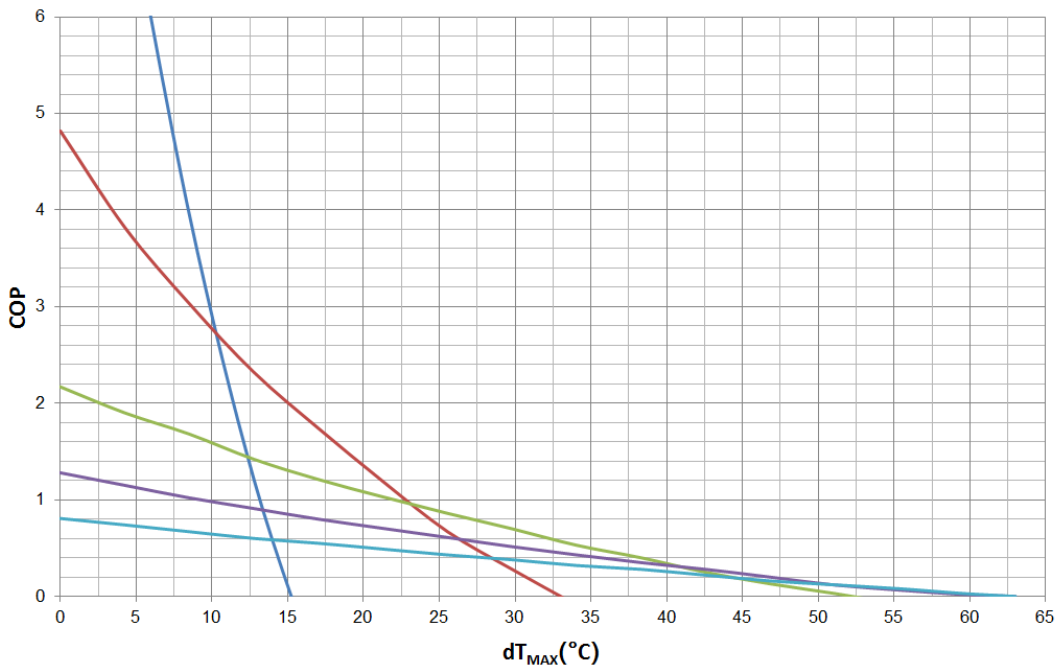
Figure 20. COP vs. dT_{MAX}
