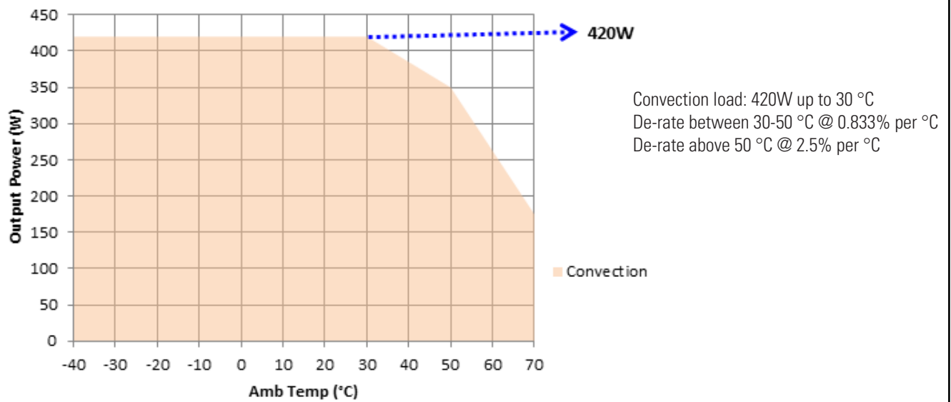
Derating Curve 24 V & above for slotted cover
