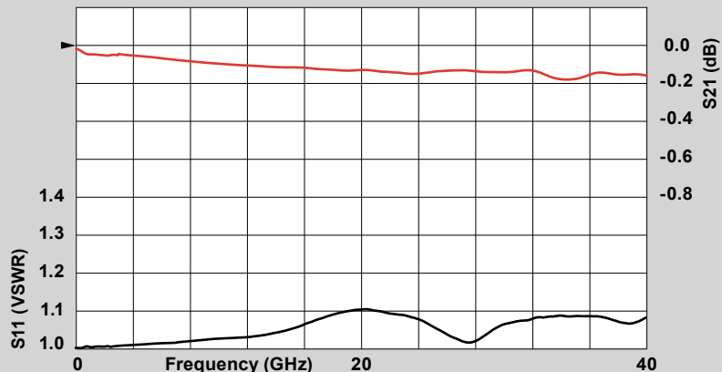
Connector: FRF40-001 Tested as back-to-back pair
