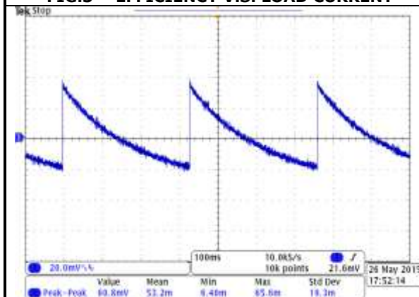
FIG.5 OUTPUT RIPPLE (12VIN, 1VOUT, IOUT=0A)
