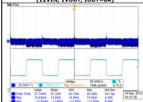
FIG.7 TRANSIENT RESPONSE (12VIN, 1VOUT, 50% to 100% LOAD STEP)
