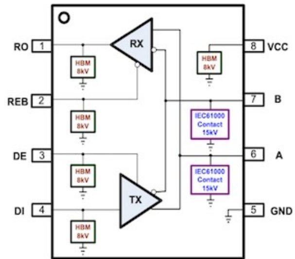
Functional Block of AZRS3072
