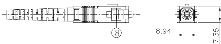
SC drawing
