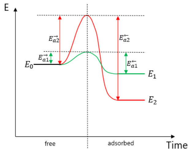
Figure 6. Schematic representation of the energy levels of two different H 2 O adsorption sites in the sensing polymer, where the green path represents absorption and desorption (forward and backward reaction) in common states with a low energy barrier and small energy difference between the occupied E_1 and unoccupied E_0 state. The red path represents the same absorption and desorption processes in extraordinary sites, exhibiting a significantly higher energy barrier and a lower energy of the adsorbed state. E_{a1,2}^{\rightarrow} stands for the activation energy needed for a water molecule to adsorb and E_{a1,2}^{\leftarrow} to desorb from the polymer.
