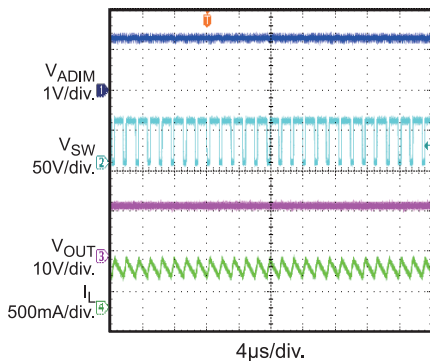
Analog Dimming
