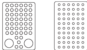
47T2 (47) #20 (2) #8 Twinax
