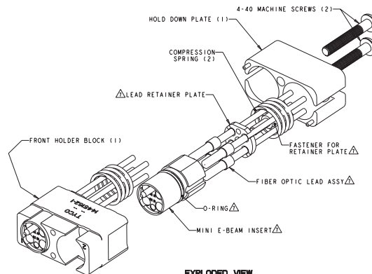
EXPLODED VIEW SCALE 3:1
