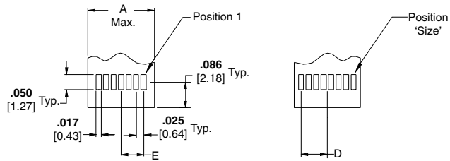
Flex Top View Size 15 shown for reference
