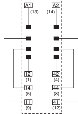
Terminal Arrangement/ Internal Connection Diagram (TOP VIEW)
