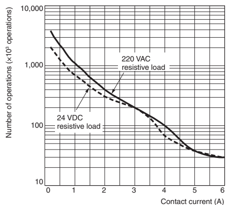
MY4□□-□□-GS-R (Resistive Load)
