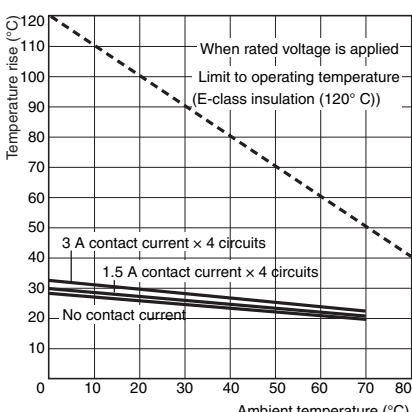
MY4□□-□□-GS-R DC Models
