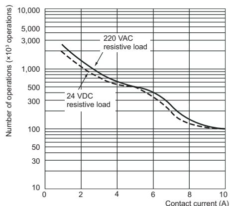
MY4□□-□□-GS-R (Resistive Load)
