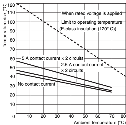
MY4□□-□□-GS-R AC Models, 50 Hz
