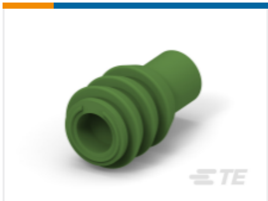
TE Part # 2287497-1 SINGLE WIRE SEAL, 1.5MM CONTACT SYSTEM
