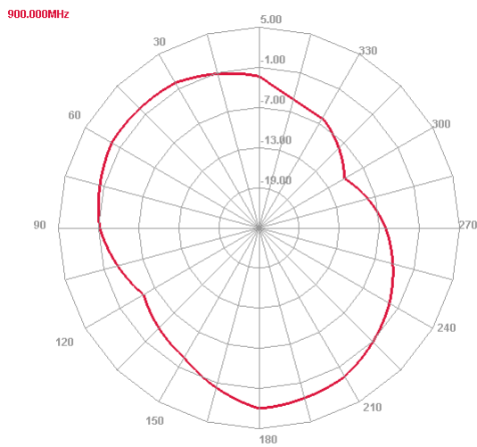
E plane
