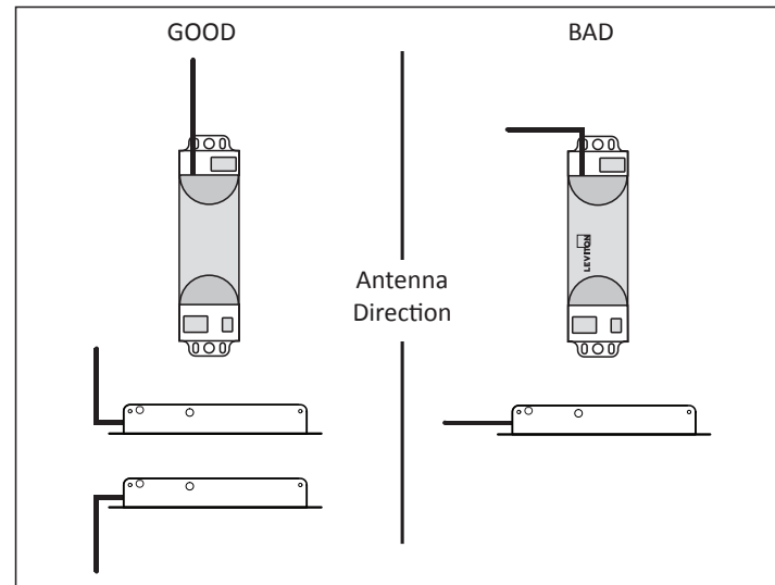
Figure 1 - Antenna Orientation
