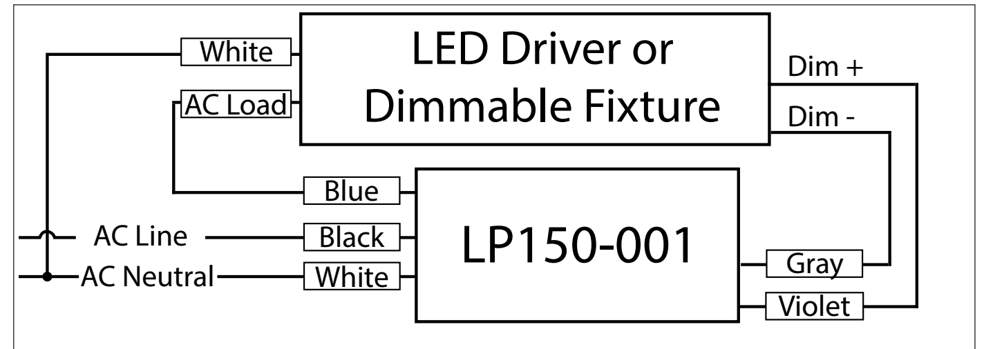
Figure 2 - Wiring Diagram
