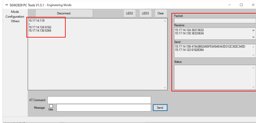
Figure 11 AT+RF_SEND Command Sent Message on Local PC Tool
