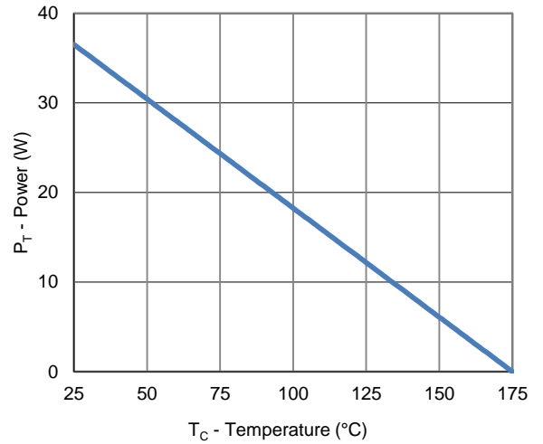
4. Power Derating
