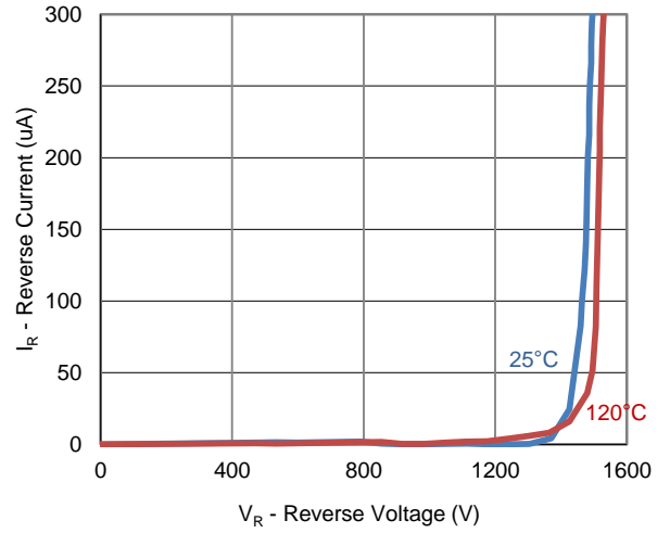
2. Reverse Characteristics
