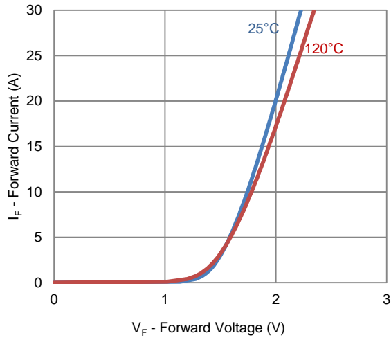
1. Forward Characteristics
