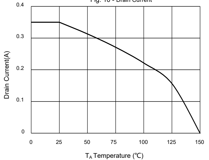
Fig. 10 - Drain Current
