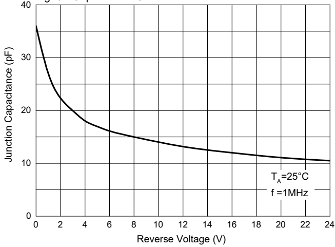
Fig. 3 - Capacitance Characteristics
