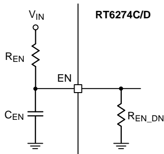
Figure 6. Automatic Start-Up Setting
